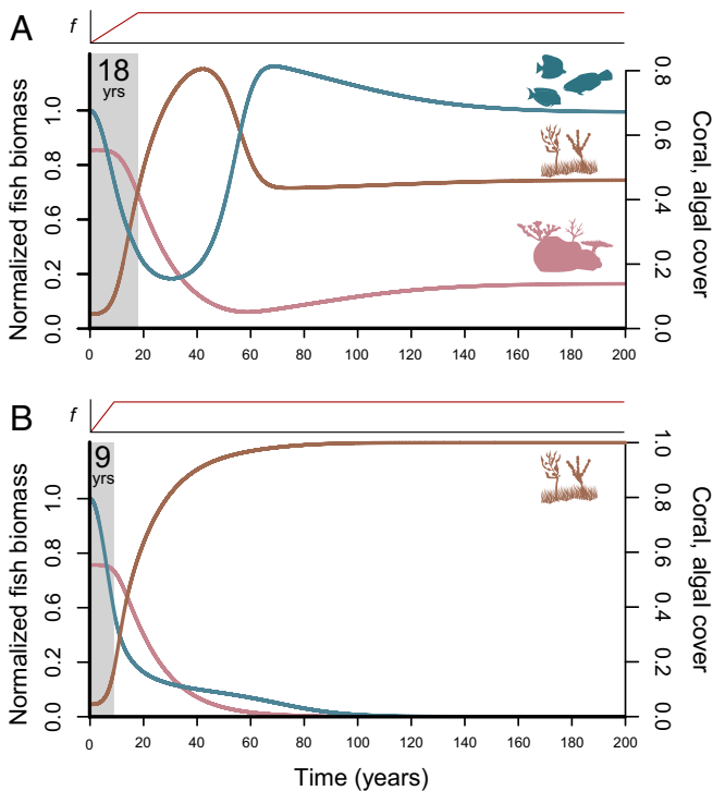
Fig. 3. Small changes in fishing effort can determine whether coral and fish populations persist or collapse. Model results illustrating a system undergoing an increase in fishing effort from no harvest ( f = 0 ) to f = 0.18 (Eq. 2). (A) Coral (pink), algae (brown), and fish (blue) population dynamics when target fishing level is reached over a period of 18 y. (B) Populations when same target harvest level is reached over a shorter period of 9 y. Slower increase in harvest (A) results in persistence of fish and coral populations; more rapid change in harvest (B) causes fish and coral population collapse.
